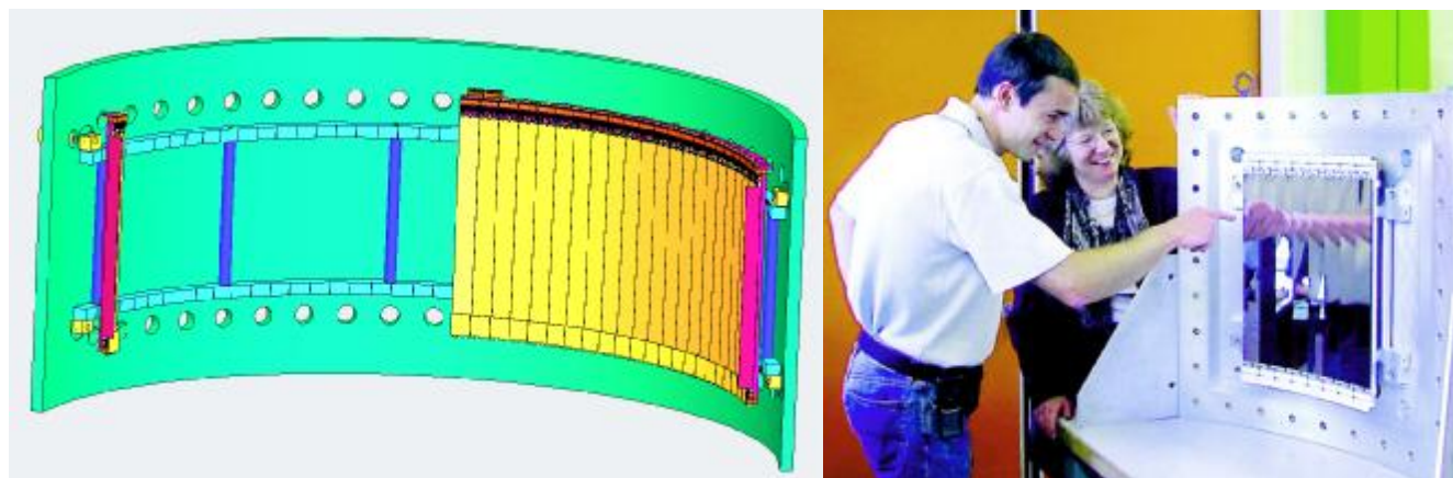
Fig. 6. The new 30°x120° 2D-PSD for D19. Large detectors match the solid angle of the best pulsed-neutron diffractometers, while benefiting from the very high flux available on the sample at a reactor source. (Guerard et al. 2002).
