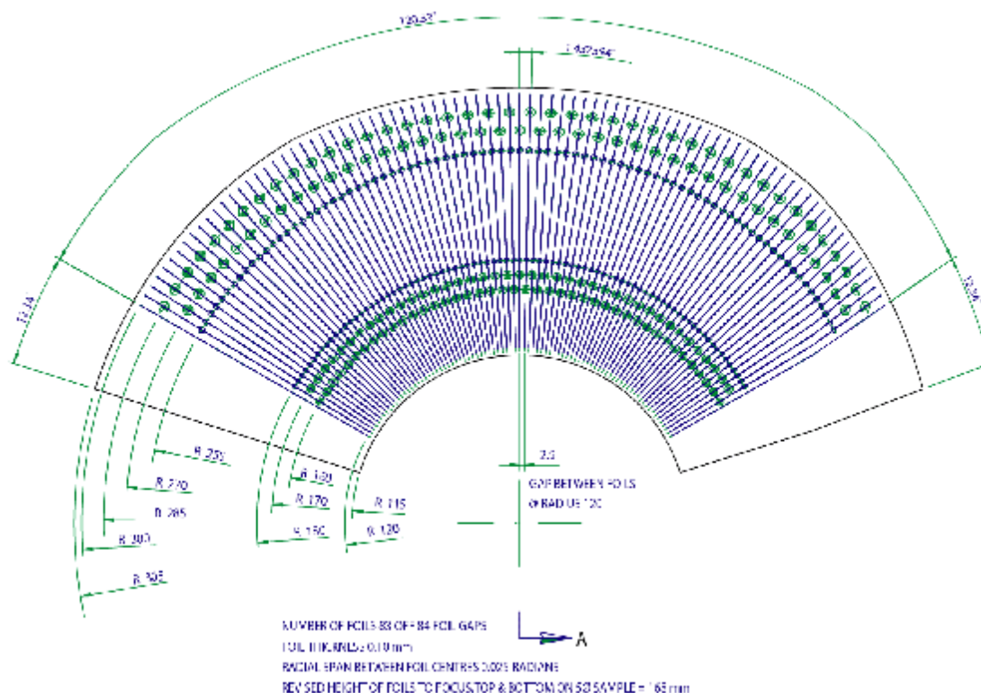
Fig.5. The Dracula radial collimator will cover a very large solid angle ( 160^\circ \times 30^\circ vertical) yet restrict scattering to a very small volume of diameter \sim 5 mm around the sample. (EuroCollimators Cheltenham, 2003).
