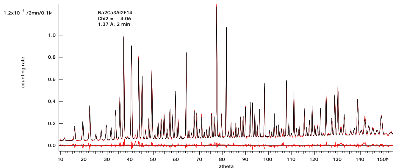
Fig. 8. Complex pattern obtained in only 2 minutes on D20 in high-resolution mode. (Hansen et al. 2003).
