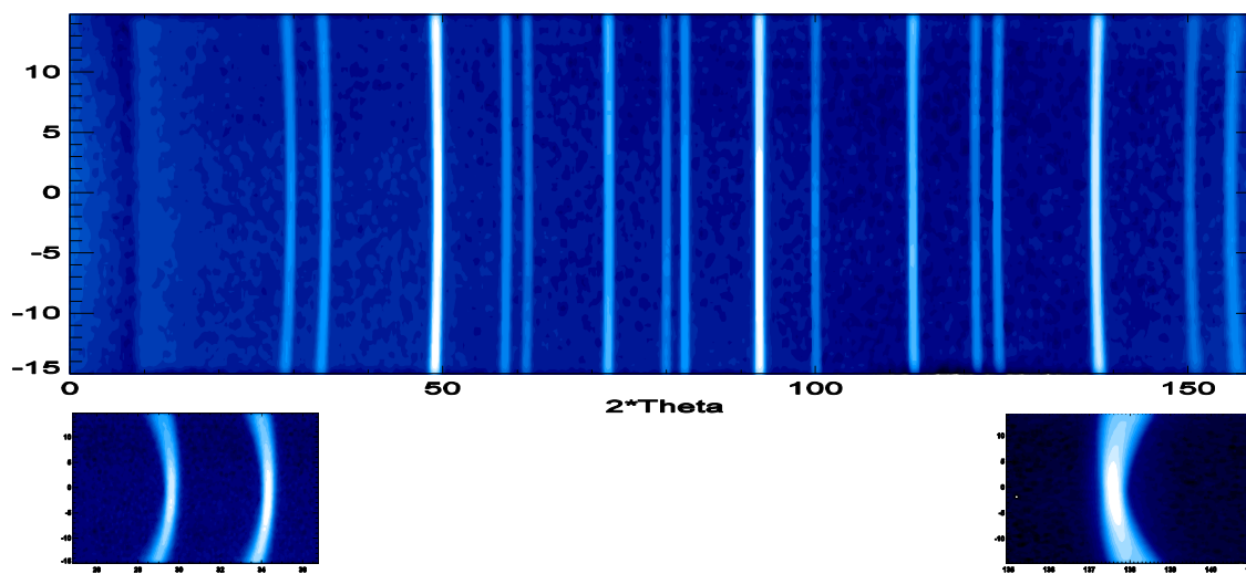
Fig. 7. High resolution powder data from a large 2D detector, showing the curvature of the diffraction cones (Suard et al 2003).
