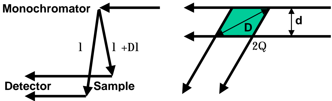
Fig. 2(a) Mosaic monochromator focussing a wide band of wavelengths 2(b) Small scattering volume with a radial collimator.
